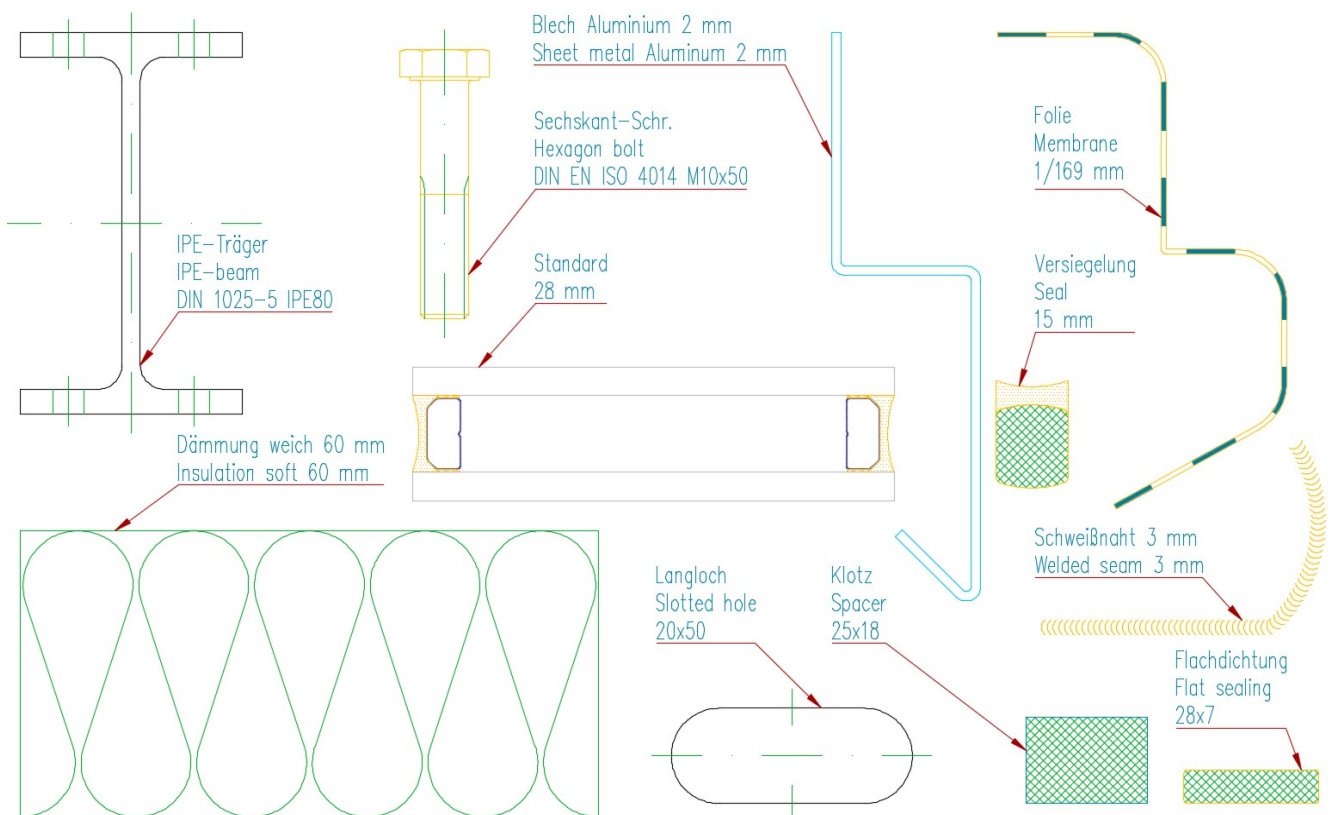
ATHENA-objects from ATHENA 2003 to 2024 in AutoCAD/LT/TrueView 2025 without ATHENA
